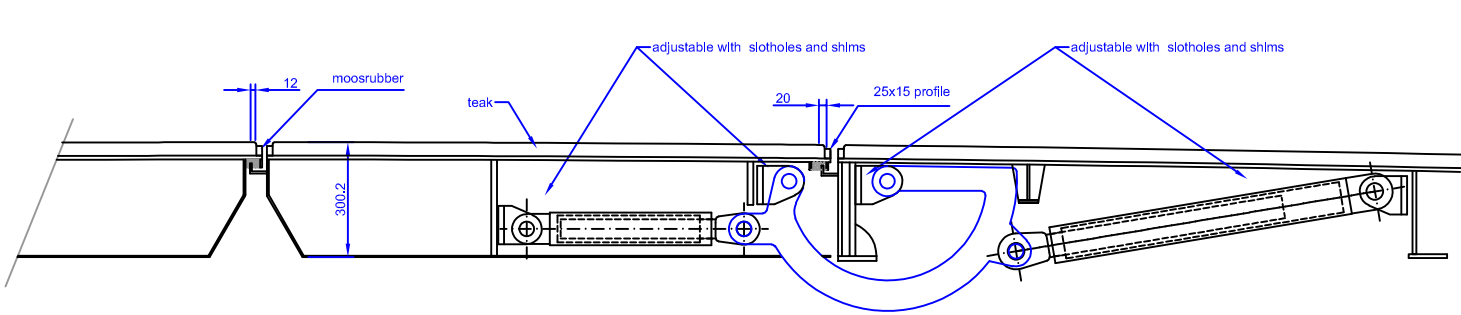
hinge and sealing details scale 1:10
